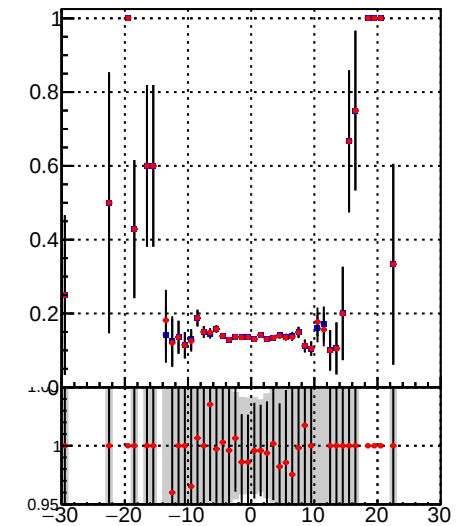
—•— DQM_TT_mkFit-DQM_lowptq_orig —•— DQM_TT_mkFit-DQM_lowptq_modi3
