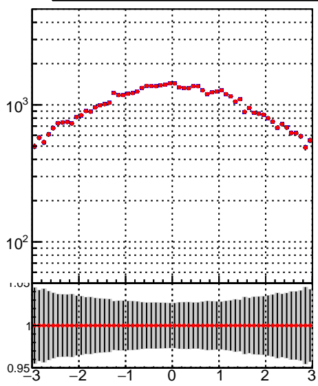
■ DQM_TT_mkFit-DQM_lowptq_orig ● DQM_TT_mkFit-DQM_lowptq_modi3
