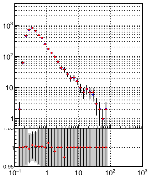
■ DQM_TT_mkFit-DQM_lowptq_orig ● DQM_TT_mkFit-DQM_lowptq_modi3
