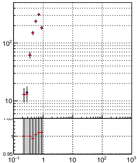
■ DQM_TT_mkFit-DQM_lowptq_orig ● DQM_TT_mkFit-DQM_lowptq_modi2
