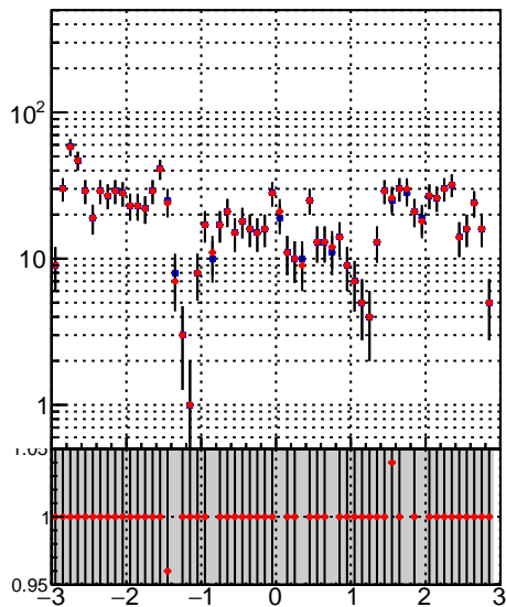
■ DQM_TT_mkFit-DQM_lowptq_orig ● DQM_TT_mkFit-DQM_lowptq_modi2
