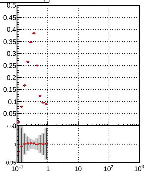
— DQM_TT_mkFit-DQM_lowptq_orig — DQM_TT_mkFit-DQM_lowptq_modi2
