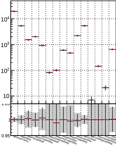
Number —●— DQM_TT_mkFit-DQM_lowptq_modi2
