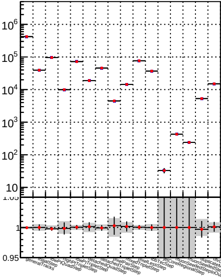
Number —●— DQM_TT_mkFit-DQM_lowptq_mc
