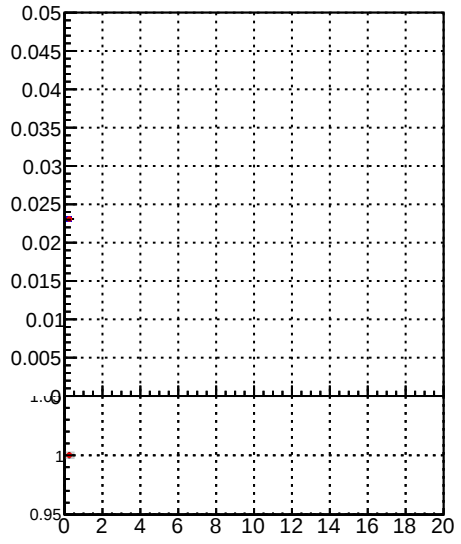
Fake rate vs. — DQM TT mkFit-DQM_lowptq_orig — DQM TT mkFit-DQM_lowptq_mod2
