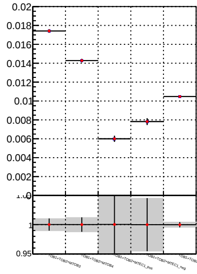
Fake rate vs. — DQM TT mkFit-DQM_lowptq_orig — DQM TT mkFit-DQM_lowptq_mod2
