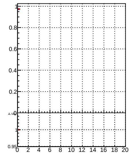
Fake rate vs. — DQM TT mkFit-DQM_lowptq_orig — DQM TT mkFit-DQM_lowptq_mod2
