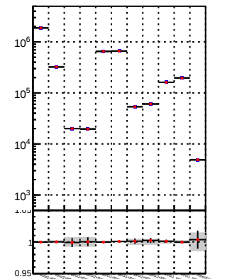
N of reco track vs. \chi^2 for different \chi^2 bins
