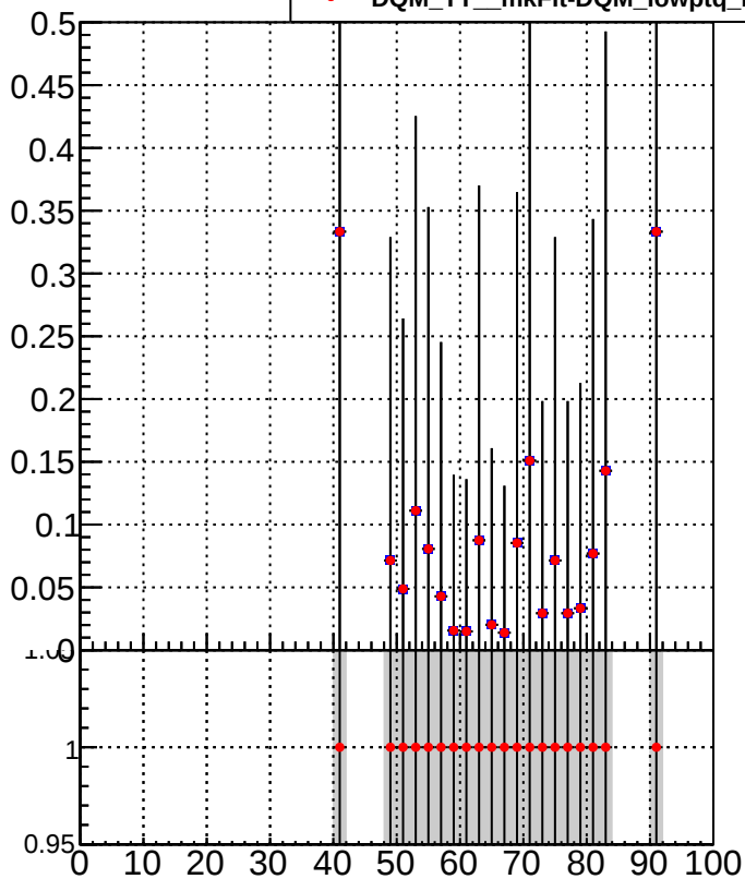
■ DQM_TT_mkFit-DQM_lowptq_orig ● DQM_TT_mkFit-DQM_lowptq_modi2
