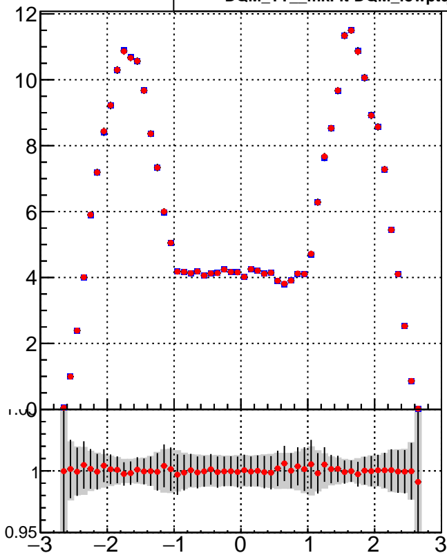
■ DQM_TT_mkFit-DQM_lowptq_orig ● DQM_TT_mkFit-DQM_lowptq_modi2
