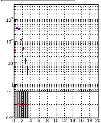
N of reco track vs. \chi^2 for DQM TT and mkFit-DQM_lowptq_modi2
