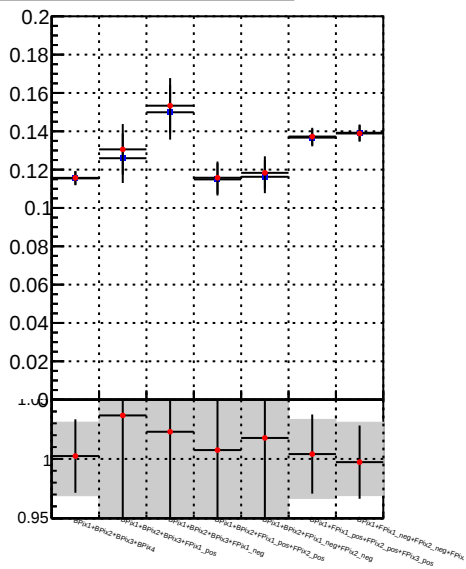
Fake rate vs. DQM_TT_mkFit-DQM_lowptq_orig DQM_TT_mkFit-DQM_lowptq_modi2
