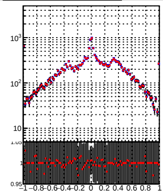
Legend: DQM_TT_mkFit-DQM_lowptq_orig (Black histogram) DQM_TT_mkFit-DQM_lowptq_modi2 (Red line with markers)
