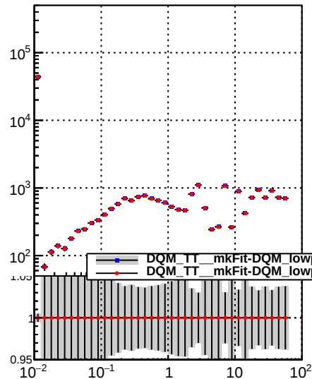
N of simulated tracks vs transverse vert position
