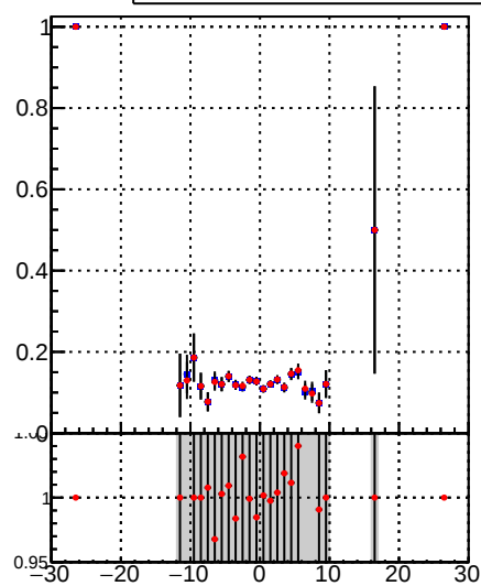
—•— DQM_TT_mkFit-DQM_lowptq_orig —•— DQM_TT_mkFit-DQM_lowptq_modi2
