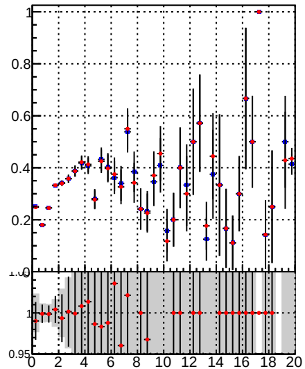
Fake rate vs. \text{mkFit-DQM\_lowptq\_orig} \text{mkFit-DQM\_lowptq\_modi2}
