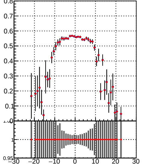
Efficiency vs. sim PV z Legend: DQM_TT_mkFit-DQM_lowptq_orig (Blue line with markers) DQM_TT_mkFit-DQM_lowptq_modi2 (Red line with markers)
