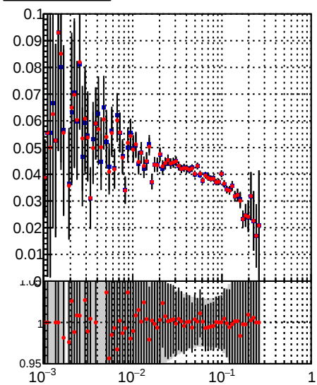
—•— DQM_TT_mkFit-DQM_lowptq_orig —•— DQM_TT_mkFit-DQM_lowptq_modi2
