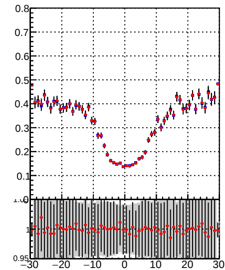
—●— DQM_TT_mkFit-DQM_lowptq_orig —●— DQM_TT_mkFit-DQM_lowptq_mod2
