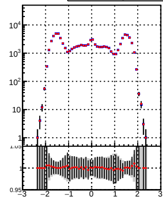
N of reco track vs \eta Legend: \bullet DQM_TT_mkFit-DQM_lowptq_orig \bullet DQM_TT_mkFit-DQM_lowptq_modi2
