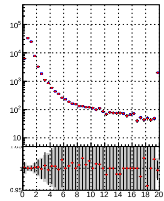
N of reco track vs. \chi^2 for DQM TT mkFit-DQM_lowptq_orig and DQM TT mkFit-DQM_lowptq_modi2
