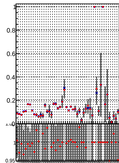
Fake rate vs. —•— DQM_TT_mkFit-DQM_lowptq_orig —•— DQM_TT_mkFit-DQM_lowptq_mod12
