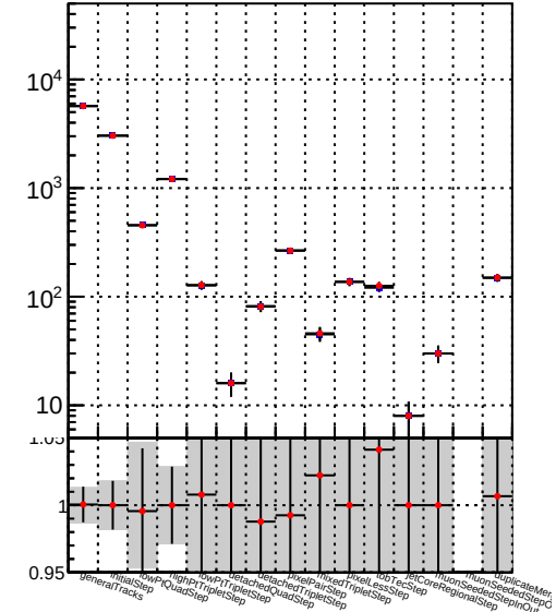
Number of tracks vs collection Legend: DQM_TT_mkFit-DQM_lowptq_orig (blue line with dots), DQM_TT_mkFit-DQM_lowptq_modi2 (red line with dots)
