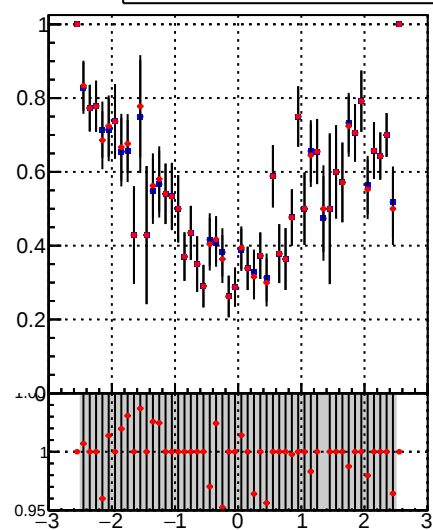
—•— DQM_TT_mkFit-DQM_lowptq_orig —•— DQM_TT_mkFit-DQM_lowptq_modi2
