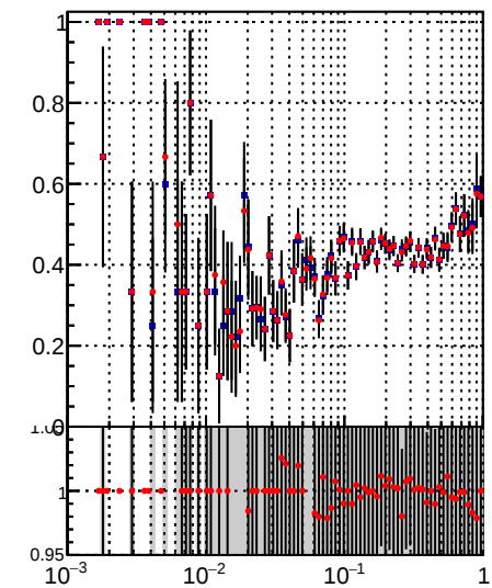
Fake rate vs dr Legend: DQM_TT_mkFit-DQM_lowptq_orig DQM_TT_mkFit-DQM_lowptq_modi2
