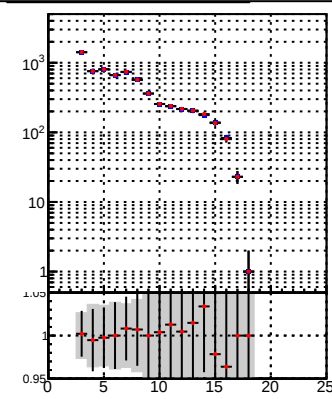
■ DQM_TT_mkFit-DQM_lowptq_orig —●— DQM_TT_mkFit-DQM_lowptq_modi2
