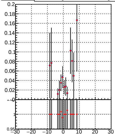
Fake rate vs vertpos DQM_TT_mkFit-DQM_lowptq_orig DQM_TT_mkFit-DQM_lowptq_modi2
