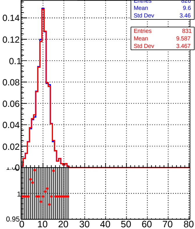
Legend: DQM_TT_mkFit-DQM_lowptq_orig (blue line with squares) DQM_TT_mkFit-DQM_lowptq_modi2 (red line with circles)
