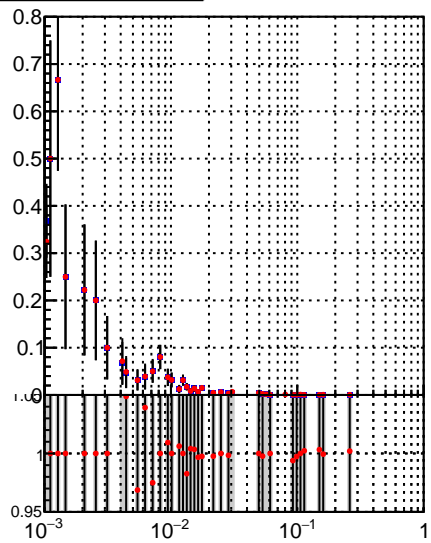
—•— DQM_TT_mkFit-DQM_lowptq_orig —•— DQM_TT_mkFit-DQM_lowptq_modi2
