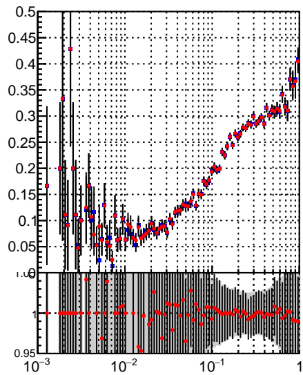
—•— DQM_TT_mkFit-DQM_lowptq_orig —•— DQM_TT_mkFit-DQM_lowptq_modi2
