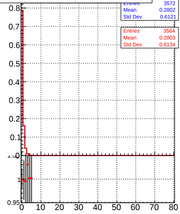
DQM_TT_mkFit-DQM_lowptq_orig DQM_TT_mkFit-DQM_lowptq_modi2
