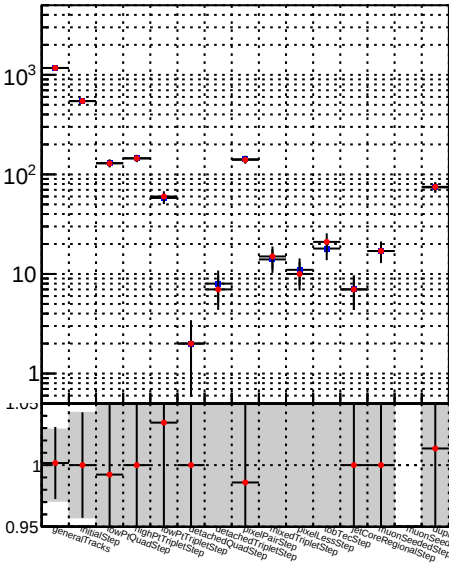
Number —●— DQM_TT__mkFit-DQM_lowptq_modi2
