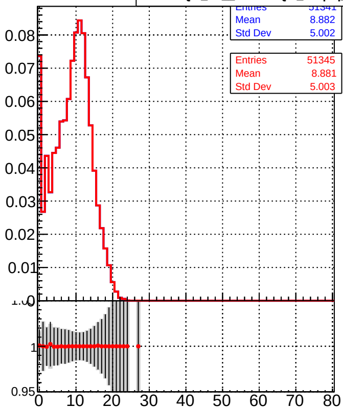
— DQM_TT_mkFit-DQM_lowptq_orig — DQM_TT_mkFit-DQM_lowptq_modi2
