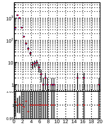
N of reco track vs. \chi^2 for DQM TT mkFit-DQM_lowptq_orig (blue) and DQM TT mkFit-DQM_lowptq_modi2 (red)
