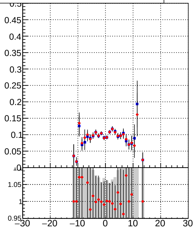
DQM_TT_mkFit-DQM_lowptq_orig DQM_TT_mkFit-DQM_lowptq_modi2
