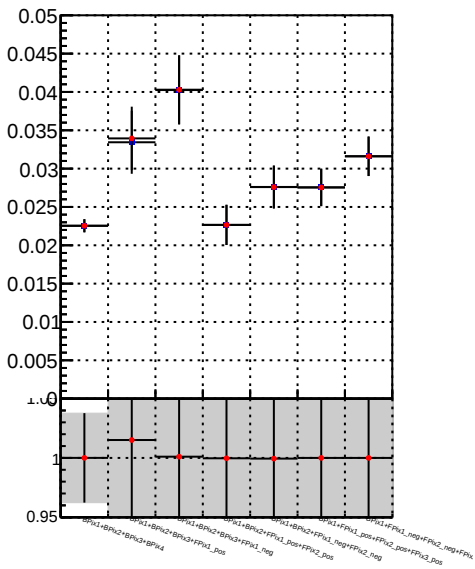
Fake rate vs. — DQM TT mkFit-DQM_lowptq_orig — DQM TT mkFit-DQM_lowptq_modi2
