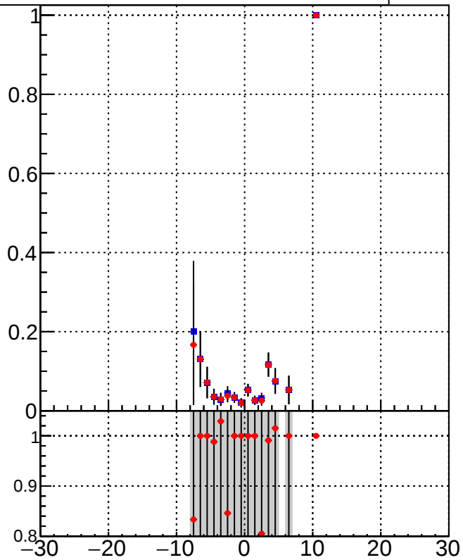
DQM_TT__mkFit-DQM_lowptq_orig DQM_TT__mkFit-DQM_lowptq_modi2
