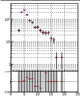
—•— DQM_TT_mkFit-DQM_lowptq_orig —x— DQM_TT_mkFit-DQM_lowptq_modi2
