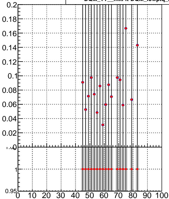
■ DQM_TT_mkFit-DQM_lowptq_orig ● DQM_TT_mkFit-DQM_lowptq_modi2
