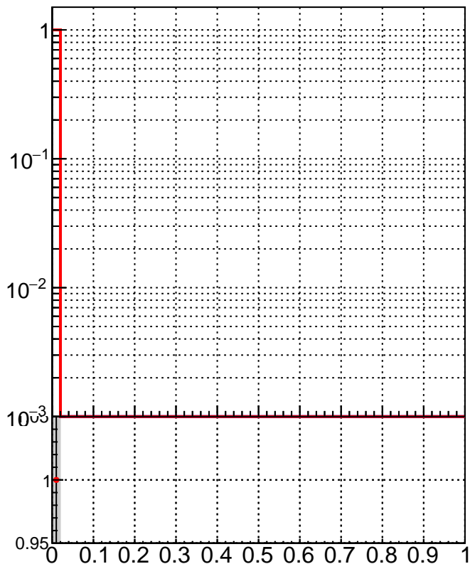
RecoPVAssoc2GenPVNotMatched_Purity
