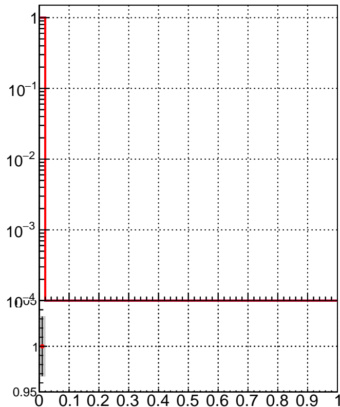
RecoPVAssoc2GenPVMatched_Purity
