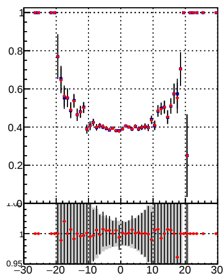
Fake rate vs d —•— DQM TT mkFit-DQM_lowptq_orig —•— DQM TT mkFit-DQM_lowptq_modi2
