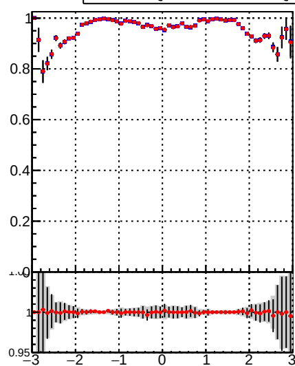
—■— DQM_TT_mkFit-DQM_lowptq_orig —●— DQM_TT_mkFit-DQM_lowptq_modi2
