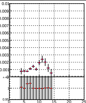
DQM_TT_mkFit-DQM_lowptq_orig
