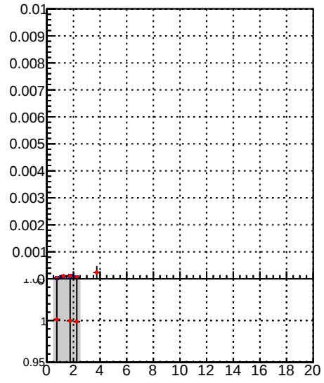
Fake rate vs. — DQM TT mkFit-DQM_lowptq_orig — DQM TT mkFit-DQM_lowptq_modi2
