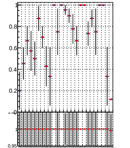
Fake rate vs. — DQM_TT_mkFit-DQM_lowptq_orig — DQM_TT_mkFit-DQM_lowptq_modi2
