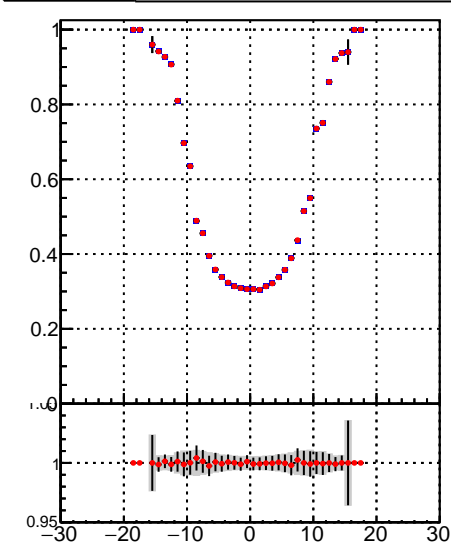
DQM_TT_mkFit-DQM_lowptq_orig DQM_TT_mkFit-DQM_lowptq_modi2
