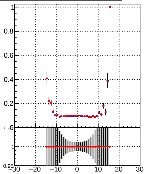
Efficiency vs. sim PV z Legend: DQM_TT_mkFit-DQM_lowptq_orig (blue line) DQM_TT_mkFit-DQM_lowptq_modi2 (red line)
