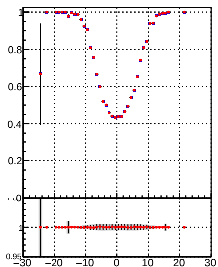
—•— DQM_TT_mkFit-DQM_lowptq_orig —•— DQM_TT_mkFit-DQM_lowptq_modI2
