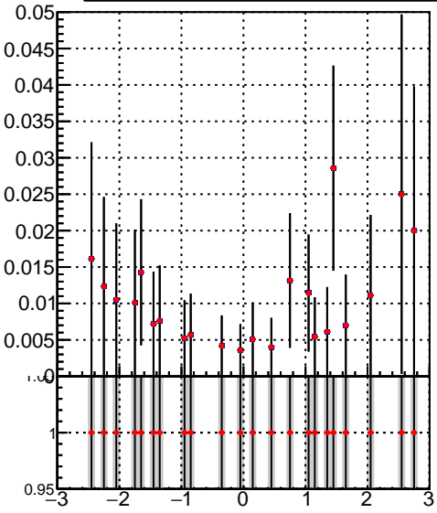
—■— DQM_TT_mkFit-DQM_lowptq_orig —◆— DQM_TT_mkFit-DQM_lowptq_modi2
