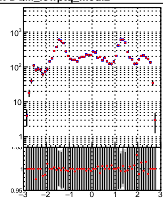
—•— DQM_TT_mkFit-DQM_lowptq_orig —•— DQM_TT_mkFit-DQM_lowptq_modi2
