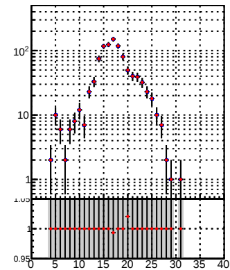
DQM_TT_mkFit-DQM_lowptq_orig DQM_TT_mkFit-DQM_lowptq_modi2
